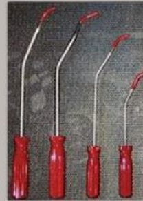
Special Valve Packing Rigid Extractor
